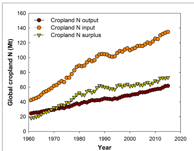
Figure 2. Global trends in crop nitrogen output, input from fertilizer and other sources, and annual nitrogen surplus (left), and map of nitrogen surplus or deficit in 2015 (top, kg N/ha). N surplus is defined as the total N input to cropland minus N harvested as crop products (15); it is expressed as million tons (Mt) in the left panel, and as kg per hectare land area in the top panel, indicating the potential pressure due to N lost from crop production. Source: Xin Zhang and Guolin Yao, University of Maryland Center for Environmental Science.
