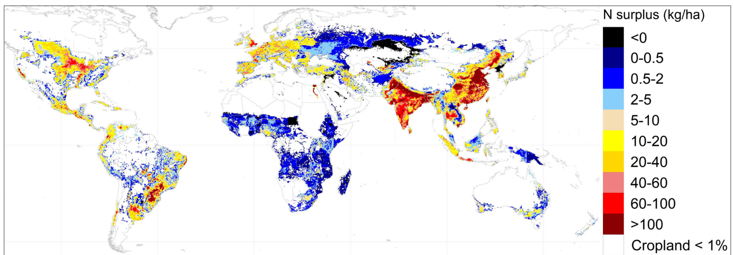
Figure 2. Global trends in crop nitrogen output, input from fertilizer and other sources, and annual nitrogen surplus (left), and map of nitrogen surplus or deficit in 2015 (top, kg N/ha). N surplus is defined as the total N input to cropland minus N harvested as crop products (15); it is expressed as million tons (Mt) in the left panel, and as kg per hectare land area in the top panel, indicating the potential pressure due to N lost from crop production. Source: Xin Zhang and Guolin Yao, University of Maryland Center for Environmental Science.
