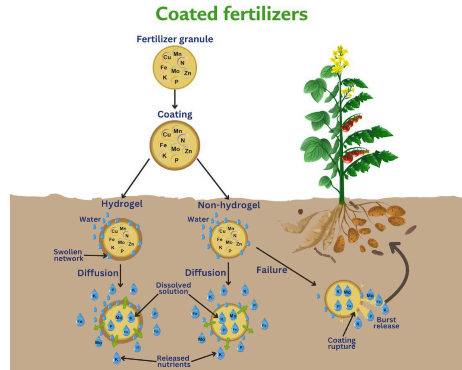
Figure 4. Mechanisms of nutrient release from coated soluble fertilizers.
